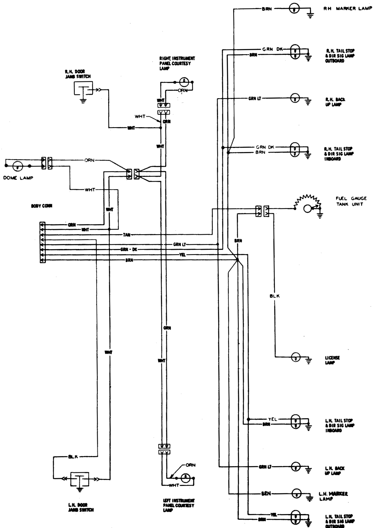
1968 Firebird Rear Lights Diagram
