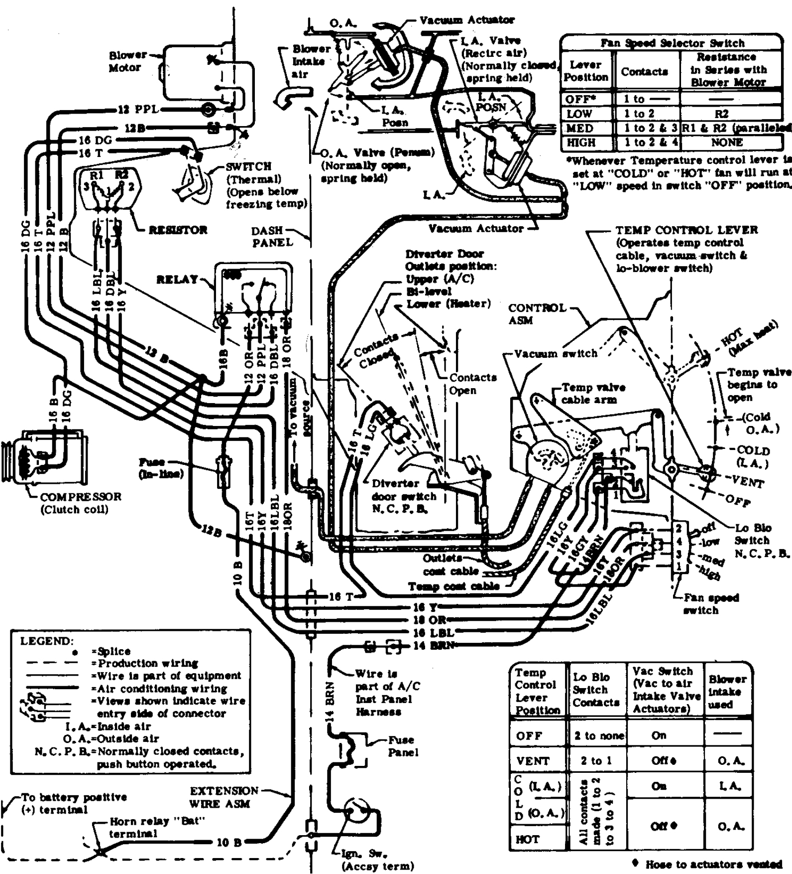
1968 FIREBIRD .. Air Conditioning & Heating Circuit
